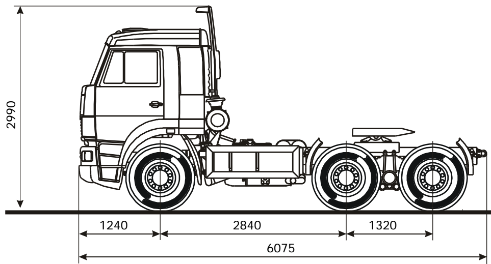
Truck dimension at curb weight The right-side steering control is available
