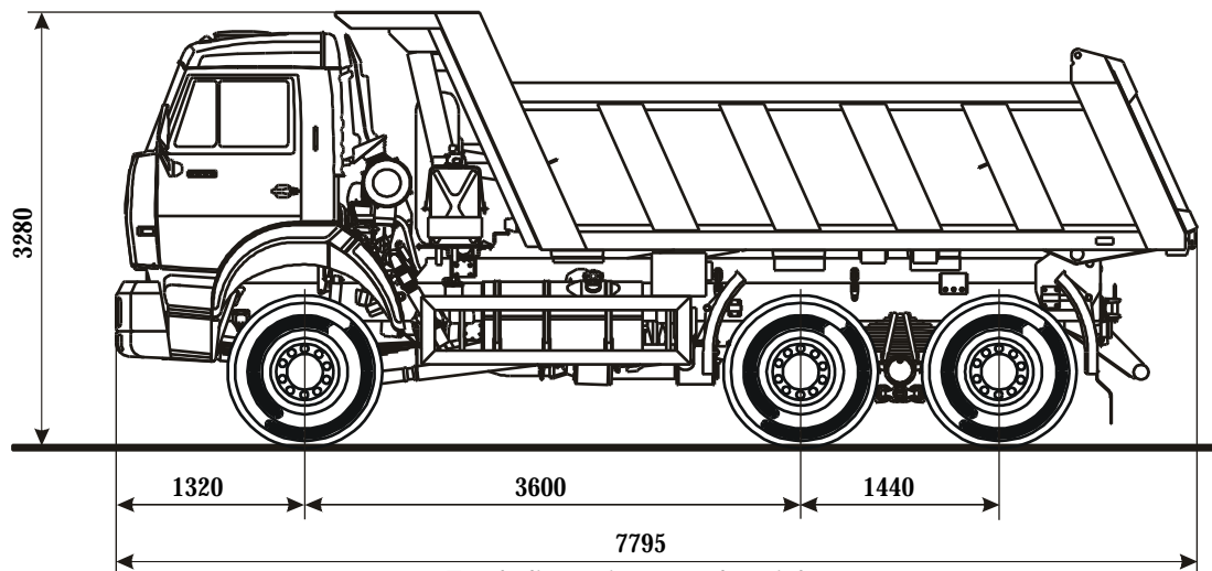
Truck dimension at curb weight The right-side steering control is available
