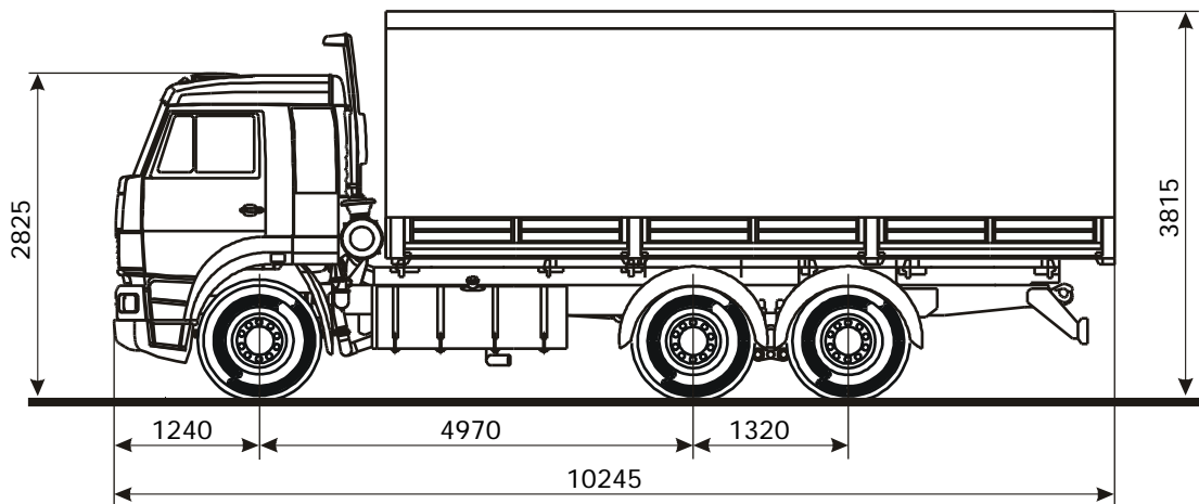
Truck dimension at curb weight
