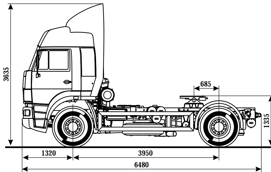
Truck dimension at curb weight
