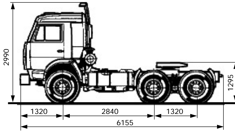
Truck dimension at curb weight
