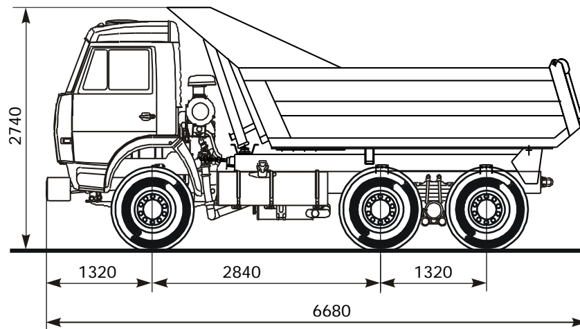
Truck dimension at curb weight
