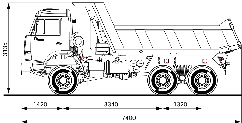
Truck dimension at curb weight
