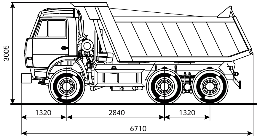
Truck dimension at curb weight
